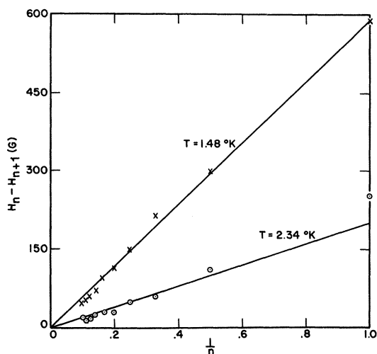
FIG. 2. Field interval between temperature spikes shown in Fig. 1 versus (1/n) . The largest spike has been designated n=1 .
