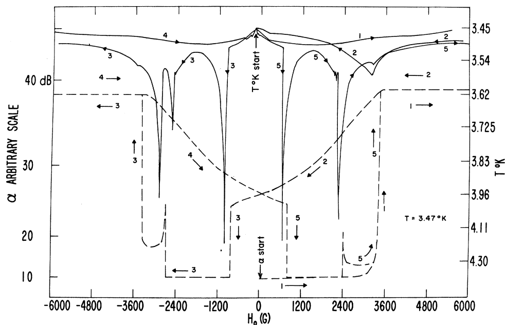
FIG. 4. Thermal (solid line) and acoustic (dashed line) hysteresis in the niobium sample No. 2 reported. The T^{\circ}\text{K} curve has been shifted to the left 0.17 kG (as shown).
