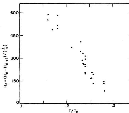
FIG. 3. Slopes H_f = (H_n - H_{n+1})/(1/n) versus reduced temperature T/T_c with T_c = 9.21 °K. The \text{He}^4 gas pressure was approximately 10 \mu .
