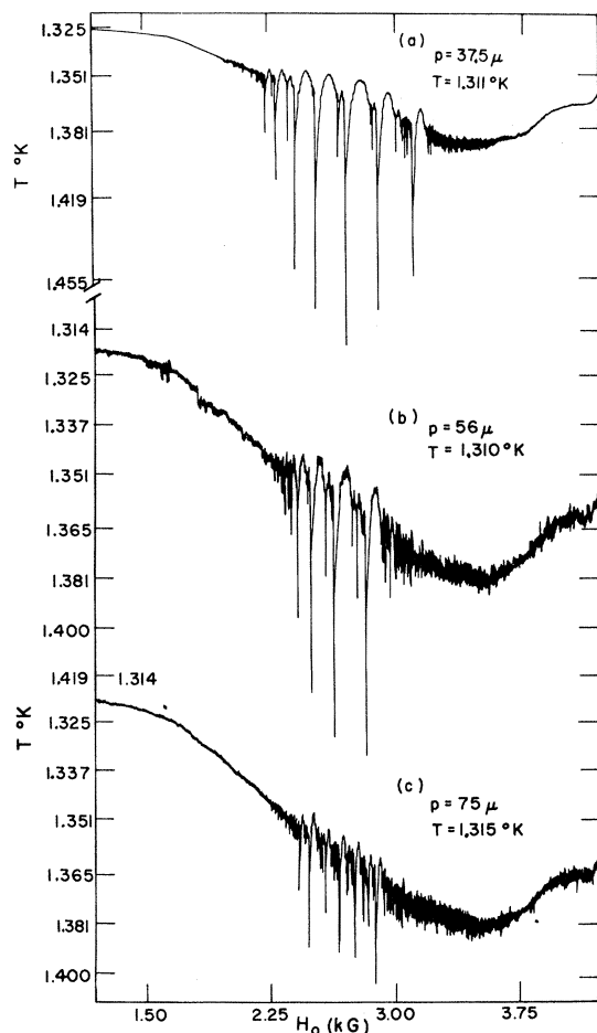
FIG. 5. Temperature spikes in niobium at different pressures, as shown. Data obtained at 10 \mu are shown in Fig. 1.
